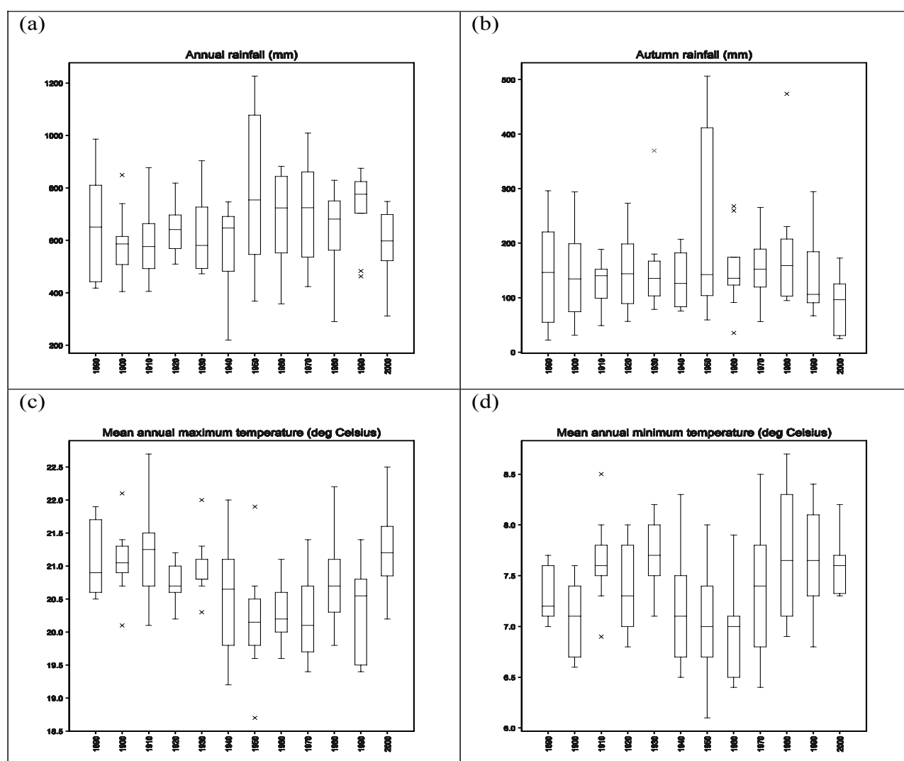
Figure 2. Box plots showing the distribution over each decade from 1890 of weather data obtained from SILO Data Drill for Yass, NSW, for (a) annual rainfall, (b) autumn rainfall (1 Mar-31 May), (c) annual average maximum and (d) minimum temperatures. The boxes show the middle 50% of values, the lines extending above and below the boxes show the upper and lower 25% of values. Extreme values (outliers) are shown by symbols. The line inside each box shows the median (middle) value.
