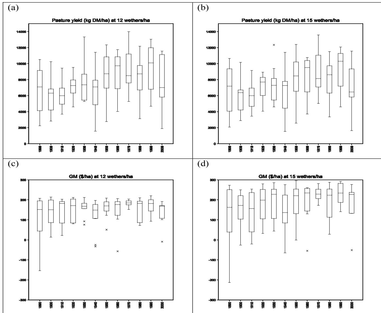
Figure 3. Box plots showing the distribution over each decade from 1890 of annual pasture yield and annual gross margin (GM) from simulations of a fine wool wether flock stocked at either (a and c) 12 or (b and d) 15 wethers/ha. The boxes show the middle 50% of values, the lines extending above and below the boxes show the upper and lower 25% of values. Extreme values (outliers) are shown by symbols. The line inside each box shows the median (middle) value.
